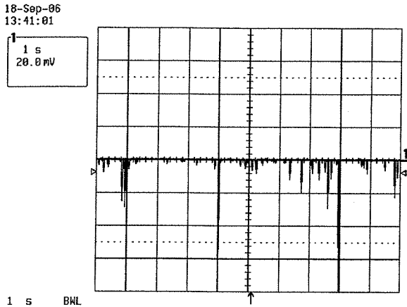
figure 2 The trace for a 5" 9390B operated at 5 \times 10^5 gain. The oscilloscope sensitivity is 20 mV/cm and yet the number of pulses is considerably higher than those in Figure 1.
