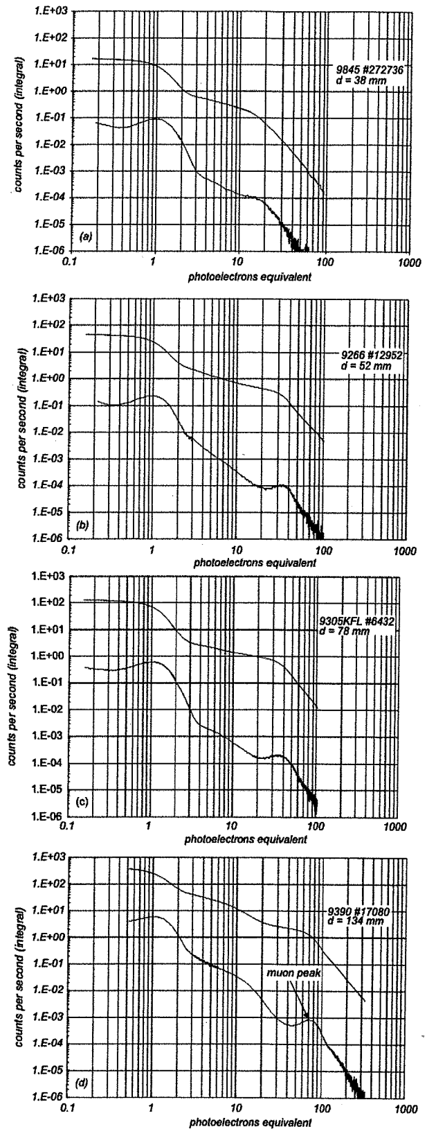
figure 3 (a) – (d) Differential and integral pulse height distributions measured for a set of photomultipliers of different window diameter, and different window thickness. Each differential curve shows a clearly resolved muon peak, except the 38 mm pmt. The integral distributions are particularly useful since they provide the expected number of counts above any stated photoelectron threshold.
